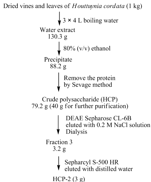
Fig. 1. Schematic diagram showing the isolation of HCP-2 from H. cordata .
