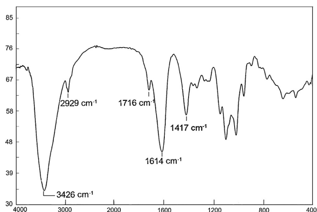
Fig. 4. FT-IR spectrum of HCP-2 in the frequency range of 400–4000 cm -1 .
