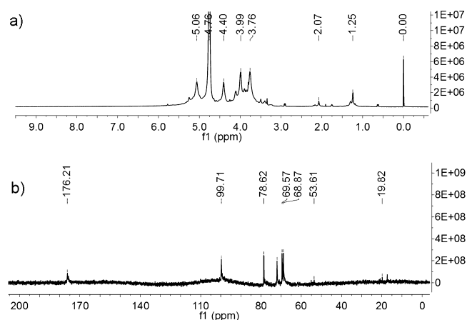
Fig. 5. (a) 1 H-NMR (D 2 O, 600 MHz) and (b) 13 C-NMR (D 2 O, 150 MHz) spectra of HCP-2.
